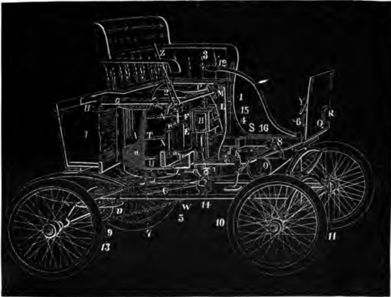
FIG. 370.—Diagram of the "Locomobile" Steam Carriage, showing parts in position. A is the boiler shell of copper; a , the winding of steel piano wire; B, the double cylinder engine; C, the adjustable strut, or distance rod; D, the compensating gear; E, pipe leading from engine to muffler, F, for exhaust steam; G, pipe leading from muffler to vent at H; I, the water supply tank; J, feed pump operated from the engine cross-head; K, cock in front of check valve on water supply pipe, for cutting off the supply from the tank; L, pipe leading from pump to the by-pass, M; N, lever for operating the by-pass; O, fuel supply tank; P, reserve air tank; Q, the dashboard; R, the air-pressure gauge; S, pipe leading from fuel tank to burner, through which gasoline is passed under air pressure; T, metal straps holding the lagging, U, around the boiler; A; V, the diaphragm fuel feed regulator, explained in connection with Fig. 207; W, pipe leading steam from boiler to diaphragm of the regulator; X, the water glass; Y, the mirror for reflecting the water glass; Z, starting lever. Other parts are: The crank arm on Z acting on the lever (1); the reversing lever (2); crank arms on the reversing lever (3 and 4); the pop safety valve set at 240 pounds (5); the steam pressure gauge (6); fuel valve to main burner (7); foot pedal (8) operating band brake (9); wire wheel spokes (10); pneumatic tire (11); steering handle (12); sprocket on rear axle (13); blow-off valve (14); oil feed cup on engine cylinders (15); pipe from air tank to fuel tank (16).
